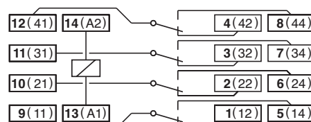
Connection diagram
