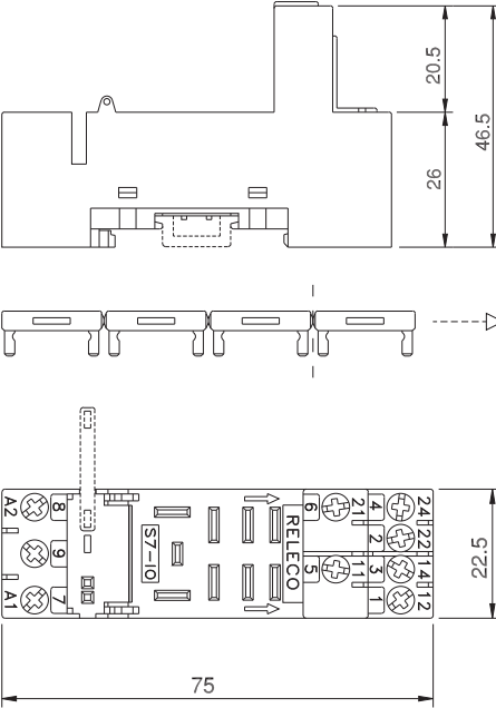
Dimensions [mm]
