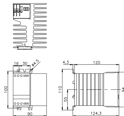
fig. 2. Dimension (mm)
