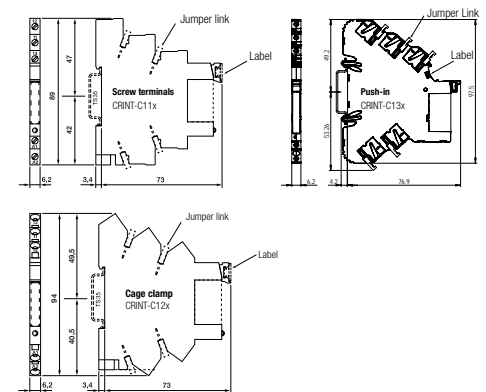
fig. 3. Dimension (mm)
