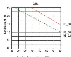
fig. 3. Thermal derating curve 40 A
