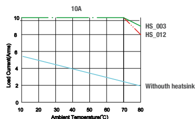
fig. 3. Thermal derating curve 15 A
