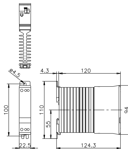
fig. 2. Dimension (mm)
