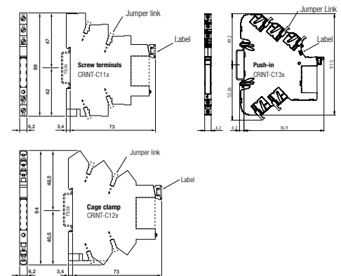
fig. 3. Dimension (mm)
