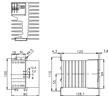
fig. 2. Dimension (mm)
