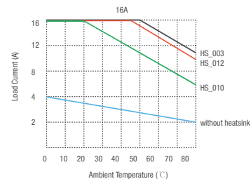
fig. 4. Thermal derating curve 25 A
