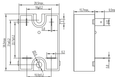
fig. 5. Dimension (mm)
