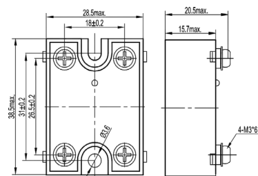
fig. 5. Dimension (mm)
