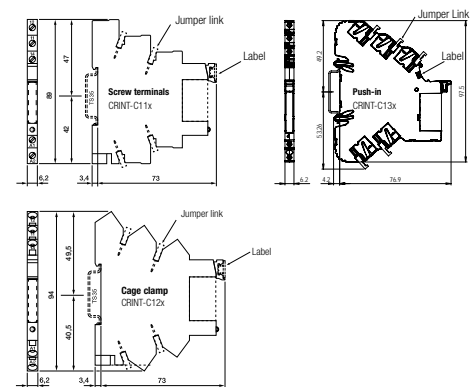
fig. 3. Dimension (mm)
