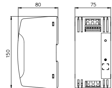
fig. 2. Dimension (mm)
