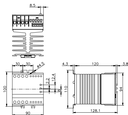
fig. 2. Dimension (mm)
