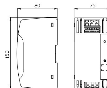
fig. 2. Dimension (mm)
