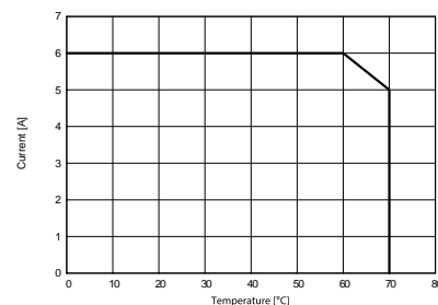
fig. 2. DC derating curve
