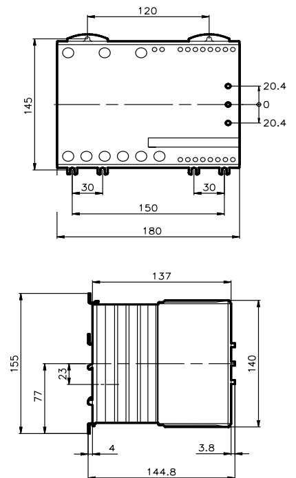
fig. 2. Dimension (mm)
