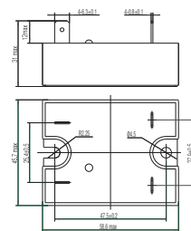
fig. 5. Dimension (mm)
