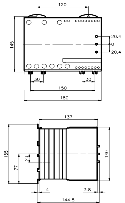
fig. 2. Dimension (mm)
