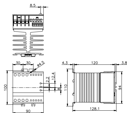
fig. 2. Dimension (mm)
