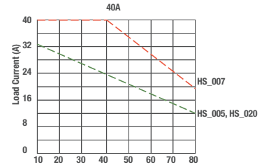
fig. 4. Thermal derating curve 60 A
