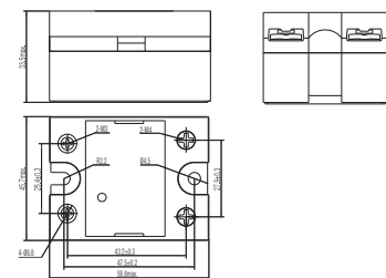
fig. 5. Dimension (mm)
