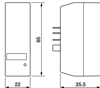
fig. 4. Dimension (mm)
