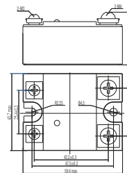
fig. 5. Dimension (mm)
