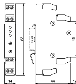
fig. 3. Dimension (mm)
