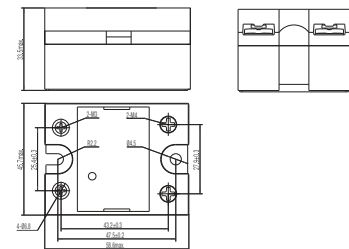
fig. 5. Dimension (mm)
