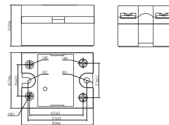
fig. 3. Dimension (mm)
