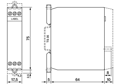
fig. 2. Dimensions (mm)
