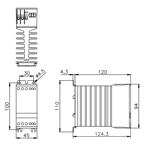
fig. 2. Dimensions (mm)
