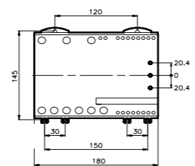
fig. 2. Dimensions (mm)
