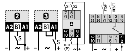
fig. 2. Dimensions (mm)
