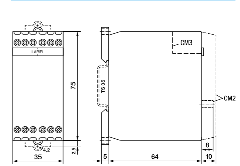
fig. 2. Dimensions (mm)
