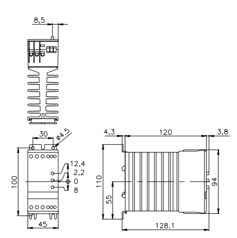
fig. 2. Dimensions (mm)
