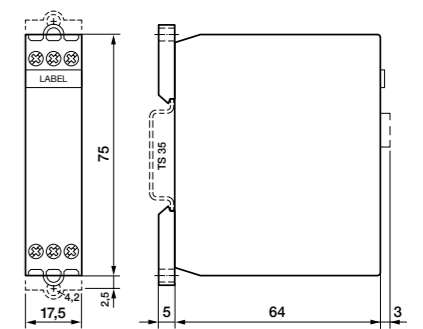
fig. 2. Dimensions (mm)
