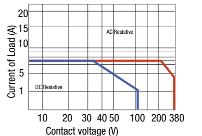
fig. 1 Max. Operating Power Curve
