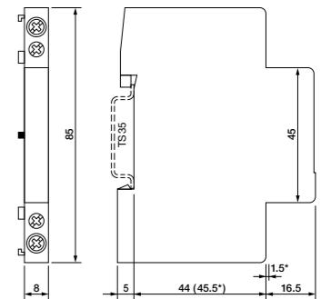
fig. 2. Dimensions (mm)
