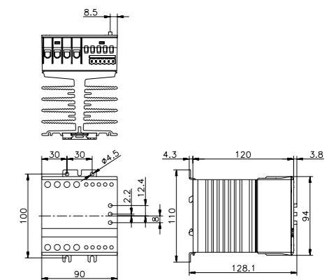
fig. 2. Dimensions (mm)
