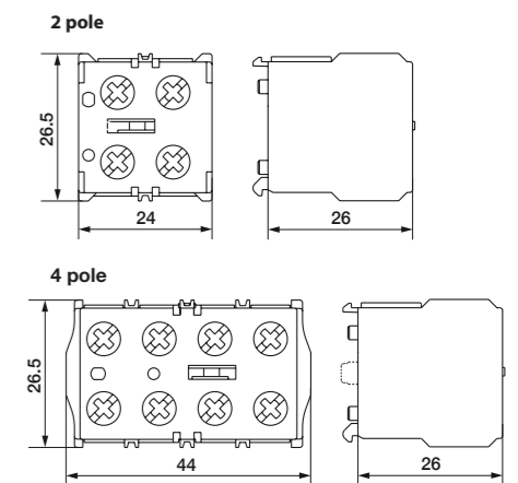
fig. 2. Dimensions (mm)
