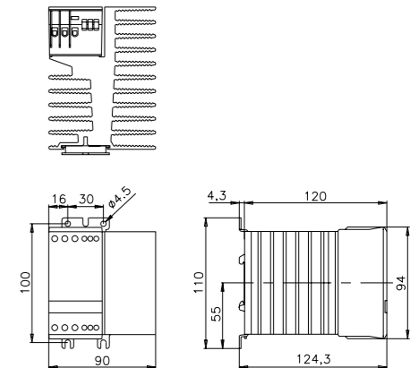
fig. 2. Dimensions (mm)
