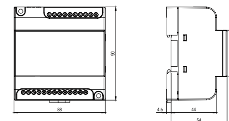
fig. 2. Dimensions (mm)
