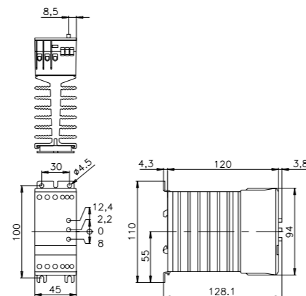
fig. 2. Dimensions (mm)
