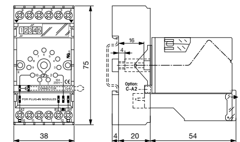
fig. 2. Dimensions (mm)
