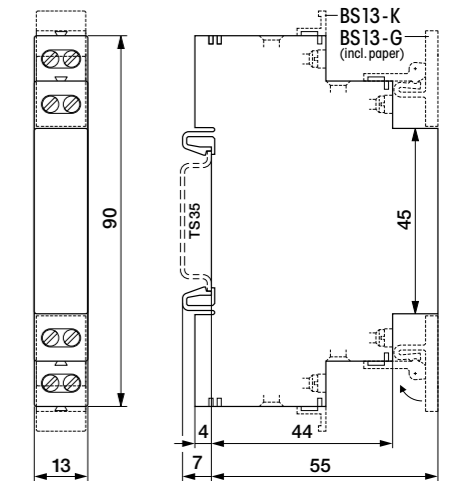
Dimension
