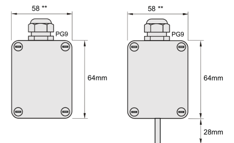
fig. 2. Dimensions (mm)
