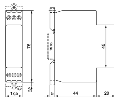
fig. 2. Dimensions (mm)
