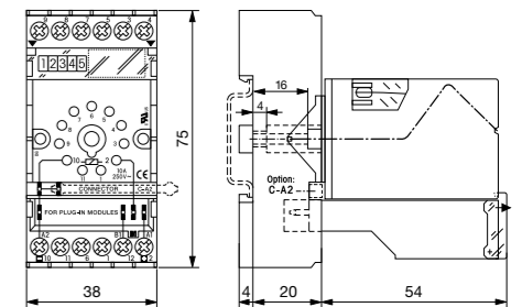
fig. 2. Dimensions (mm)
