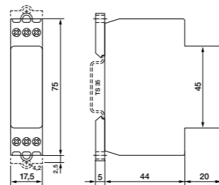
Dimensions (mm)
