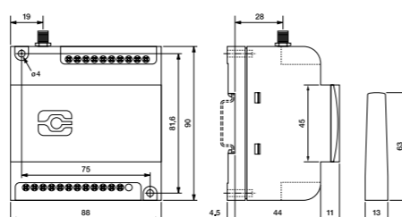
fig. 2. Dimensions (mm)
