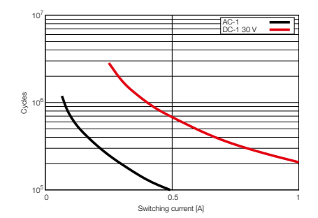
fig. 1 Contact endurance
