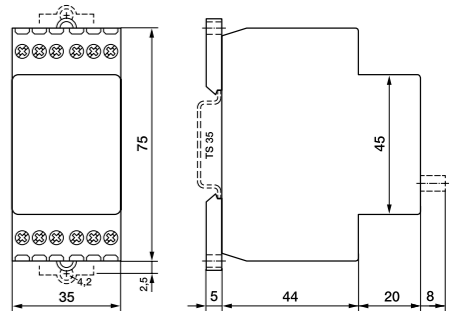
fig. 2. Dimensions (mm)
