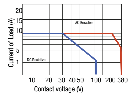
fig. 1 Max. Operating Power Curve
