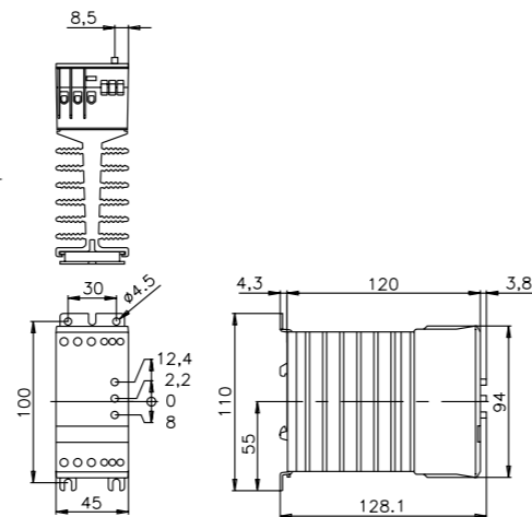
fig. 2. Dimensions (mm)
