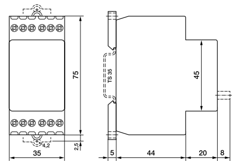
fig. 2. Dimensions (mm)
