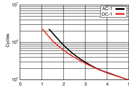
fig. 1 Contact endurance
