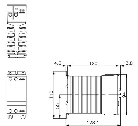
fig. 2. Dimensions (mm)
