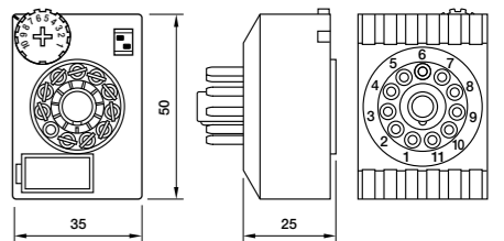
fig. 2. Dimensions (mm)
