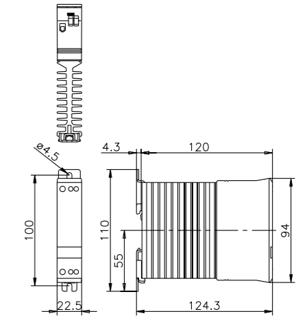
fig. 2. Dimensions (mm)
