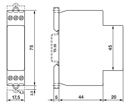
fig. 2. Dimensions (mm)
