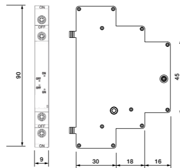
fig. 2. Dimensions (mm)
