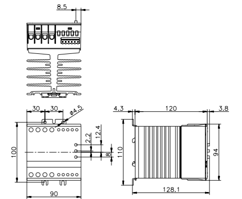
fig. 2. Dimensions (mm)
