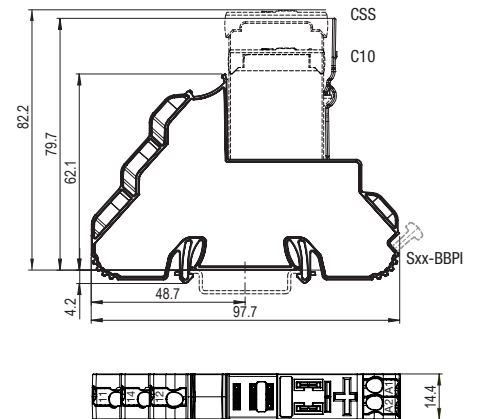
fig. 2. Dimension (mm)
