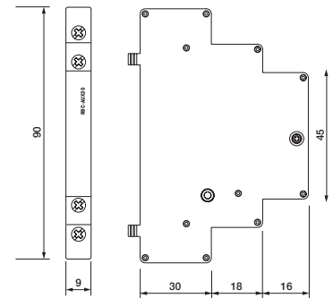
fig. 2. Dimensions (mm)
