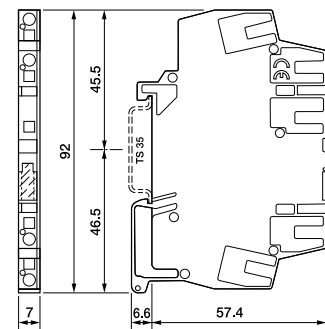
fig. 2. Dimensions (mm)
