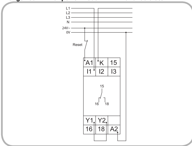
► Range 100mA with power modul 24V AC and fault latch
