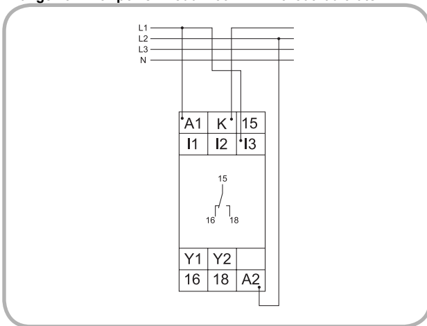
► Range 10A with power modul 400V AC without fault latch
