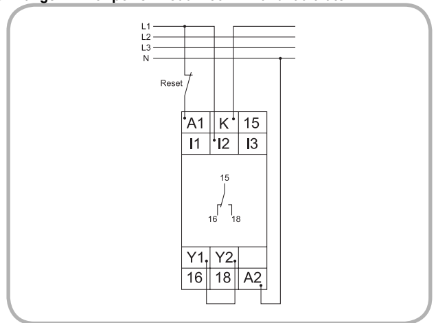
► Range 1A with power modul 230V AC and fault latch
