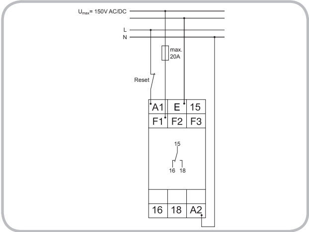
► Range 150V, supply voltage 230V AC and fault latch
