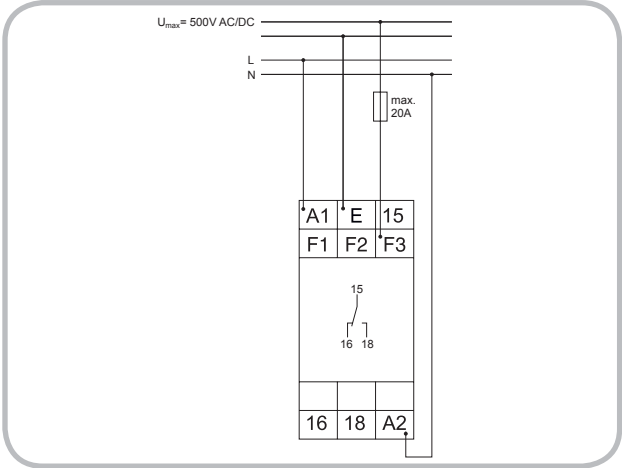
► Range 500V, supply voltage 230V AC without fault latch
