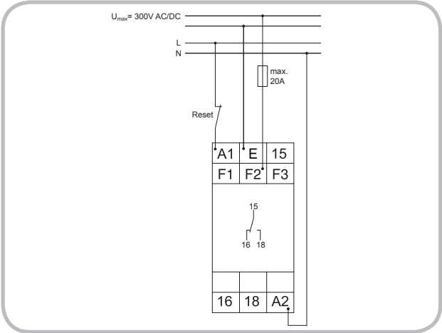
► Range 300V, supply voltage 230V AC and fault latch
